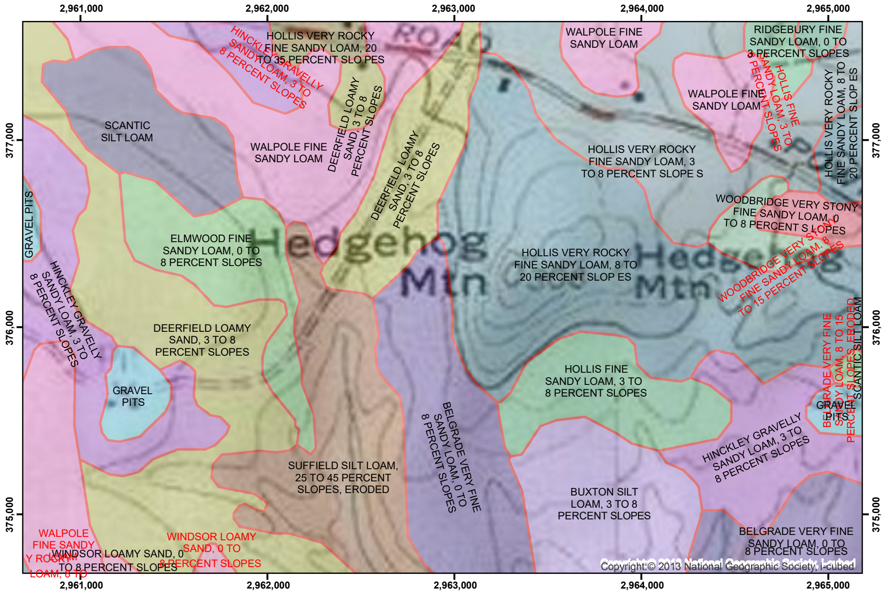
NRCS Soils in Vicinity of Hedgehog Mtn, Freeport Base Map is USGS 7.5' Quadrangle Grid is Maine State Plane, West Zone, NAD83 (ft) RG 3-22-22
